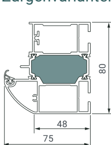
Aluminium-Zarge A3
