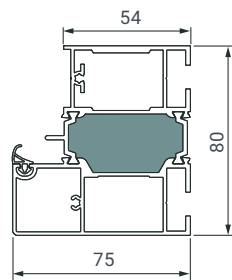
Aluminium-Zarge A4
